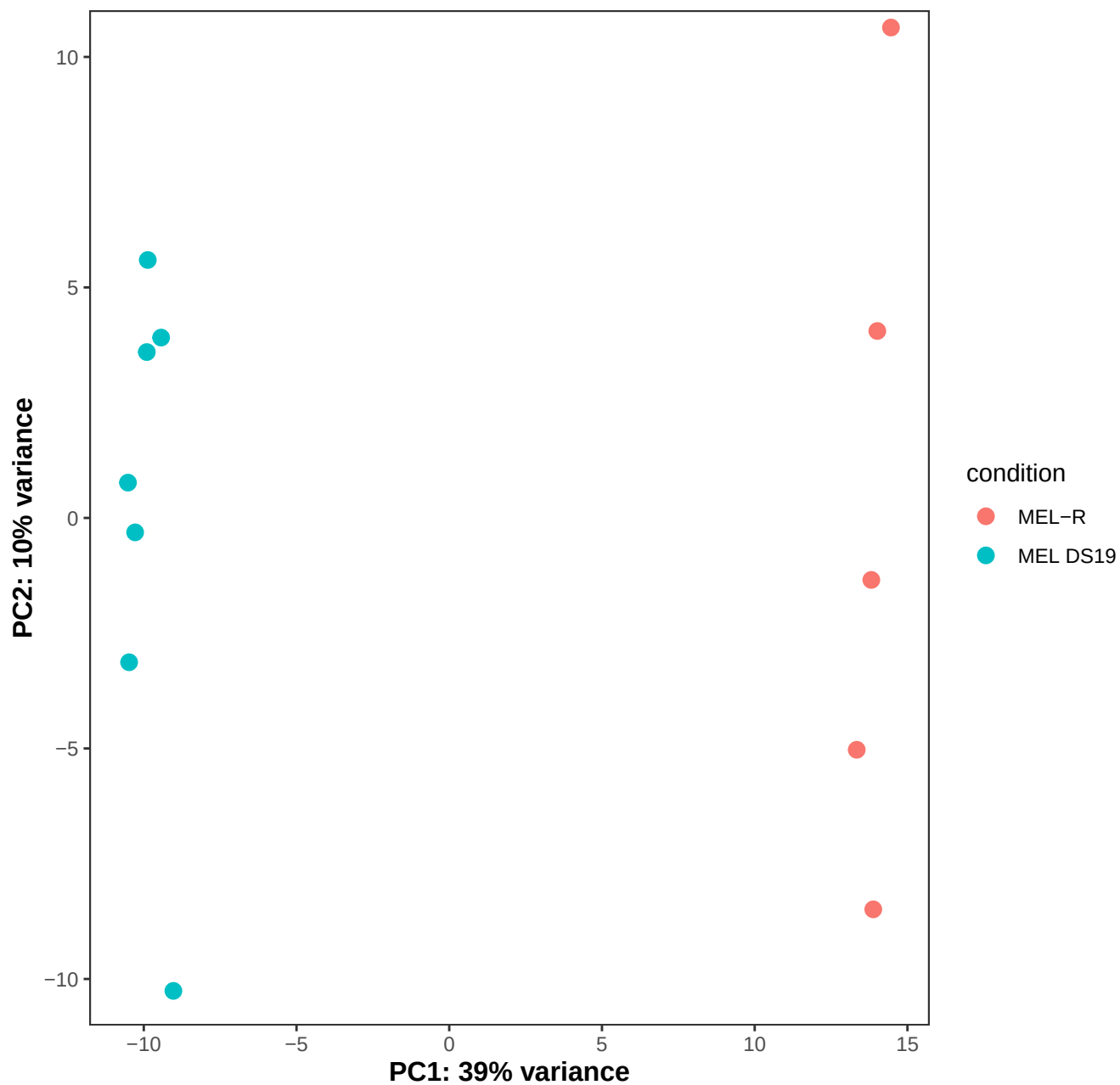
Principal Component Analysis of MEL vs MEL-R – Salmon
